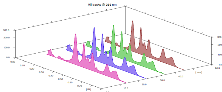
3D Peak Display of Madhumeha Kusumakar Rasa at 366 nm
