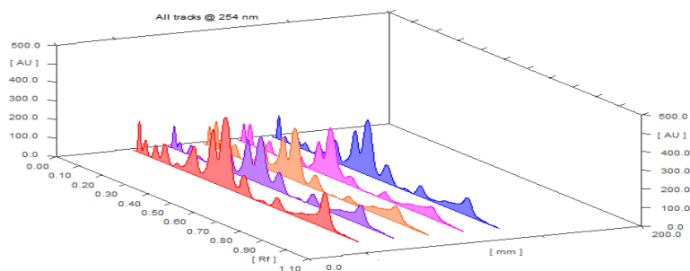
3D Peak Display of Kaishor Guggul at 254 nm
